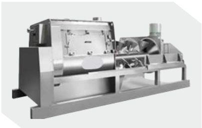
Paddle Mixer
